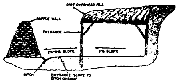
Figure 1-37. Floor and entrance drainage.
